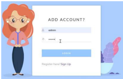
FIG 10 SIGN IN
