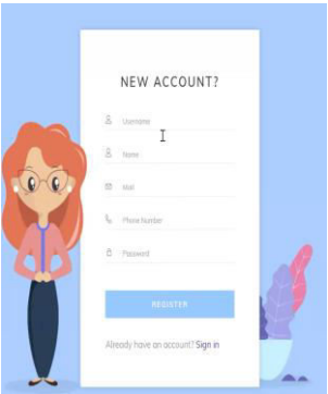
FIG 9 SIGN UP
